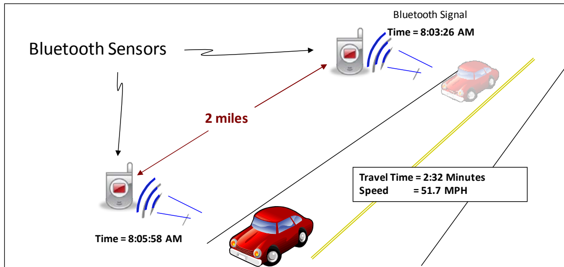
Figure 3.1: Bluetooth Data Collection Method
